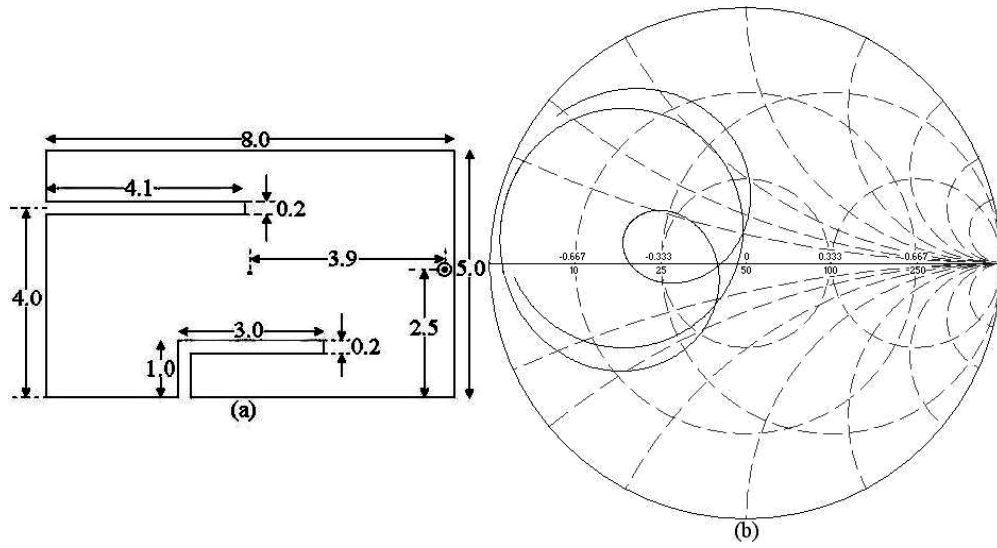
Figure 4: (a) Triple band RMSA and its (b) simulated input impedance locus
