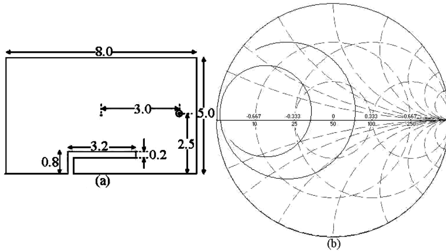
Figure 2: (a) Dual band half U-slot cut RMSA and its (b) simulated input impedance locus
