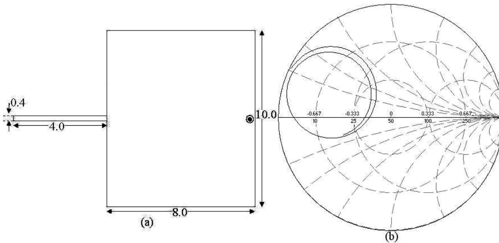
Figure 3: (a) Dual band stub loaded RMSA and its (b) simulated input impedance locus
