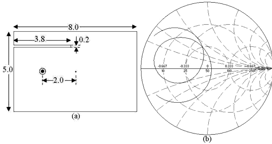
Figure 1: (a) Dual band rectangular slot cut RMSA and its (b) simulated input impedance locus
