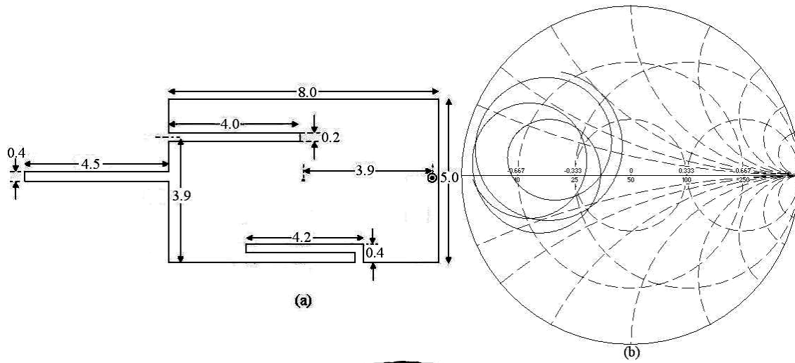
Figure 4: (a) Triple band RMSA and its (b) simulated input impedance locus
